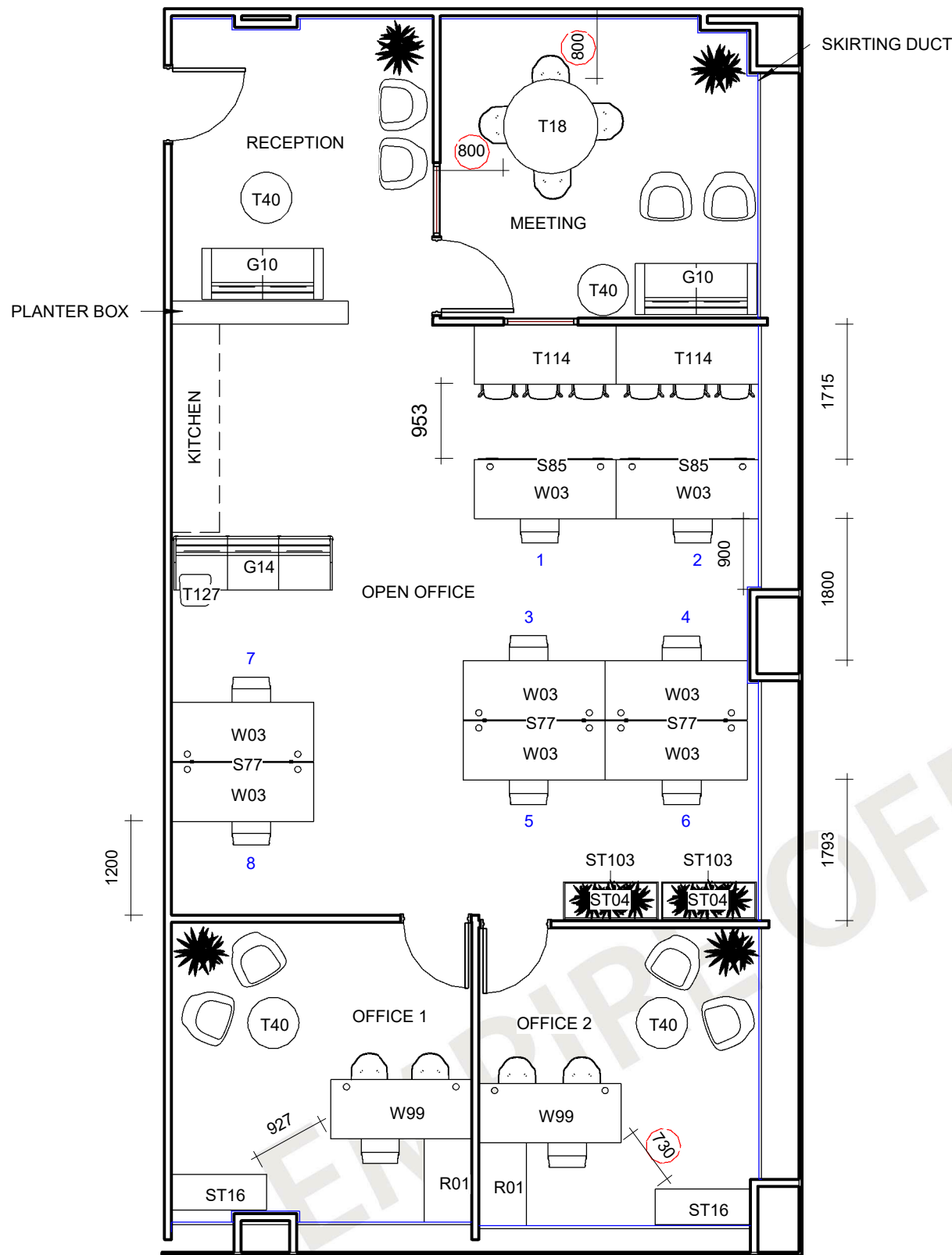
1 INSTALL DRAWING 1 : 75
