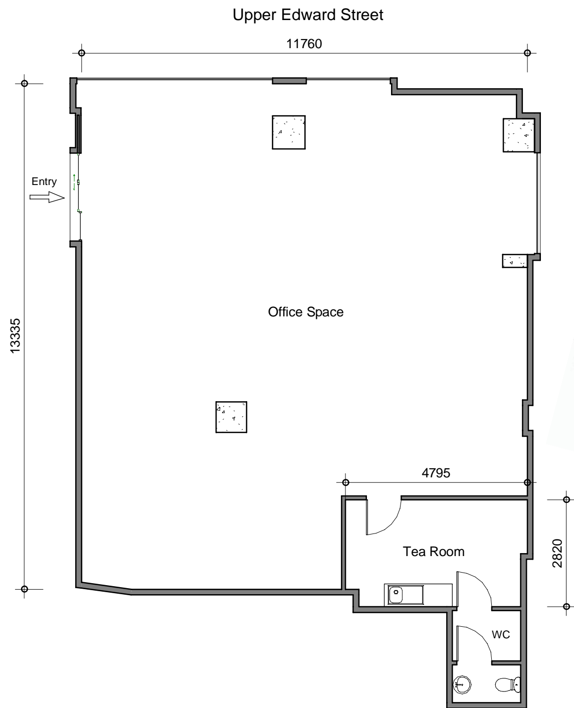
1 Ground Floor 1 : 100 Lease D Area: 161m 2
